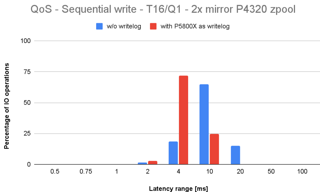
Fig. 22. Latency distribution for a sequential write test, done on a 2x 2-way mirror SSD zpool (T16/Q1), with and without writelog.
