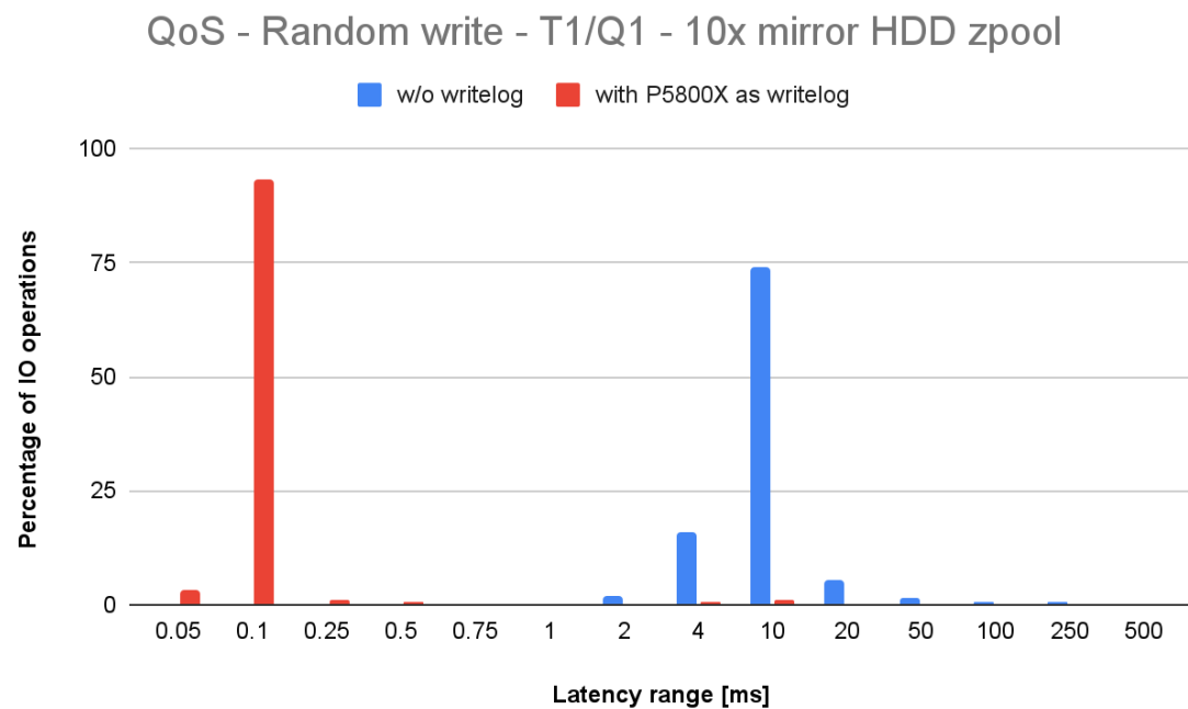
Fig. 6. Latency distribution for a random write test, done on a 10x mirror HDD zpool (T1/Q1), with and without writelog.
