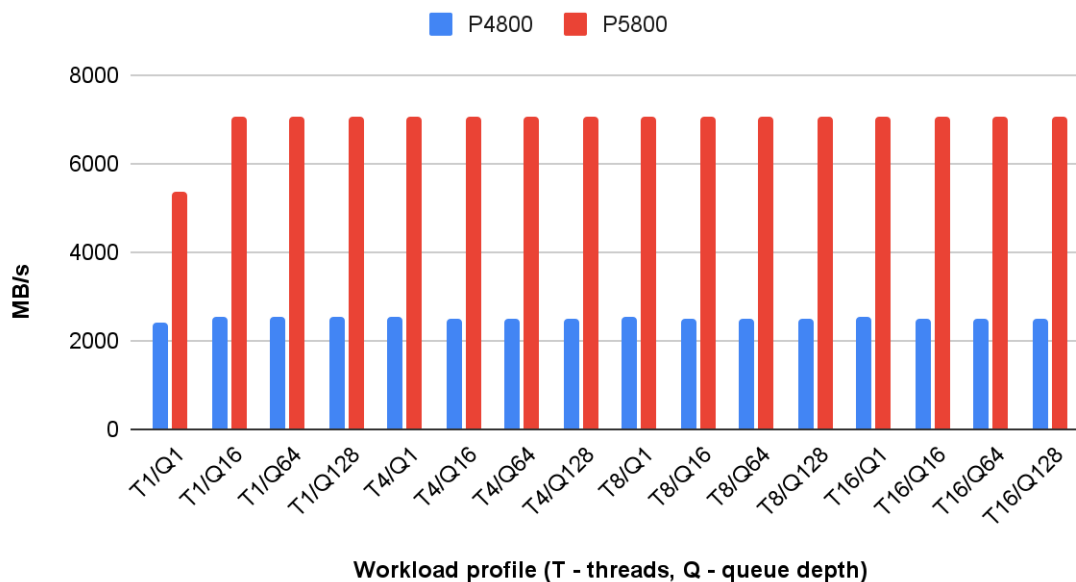
Fig. 3. Sequential read performance on raw device compared to P4800.
