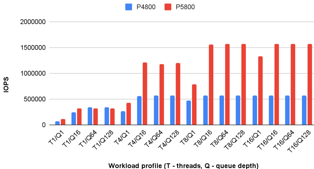
Fig. 2. Random write performance on raw device compared to P4800.
