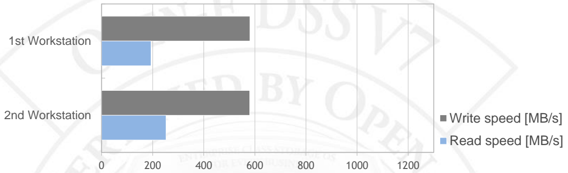
FIGURE 10: Balance-rr bonding mode performance test results chart for Myricom 10G-PCIE2-8B2-2S
